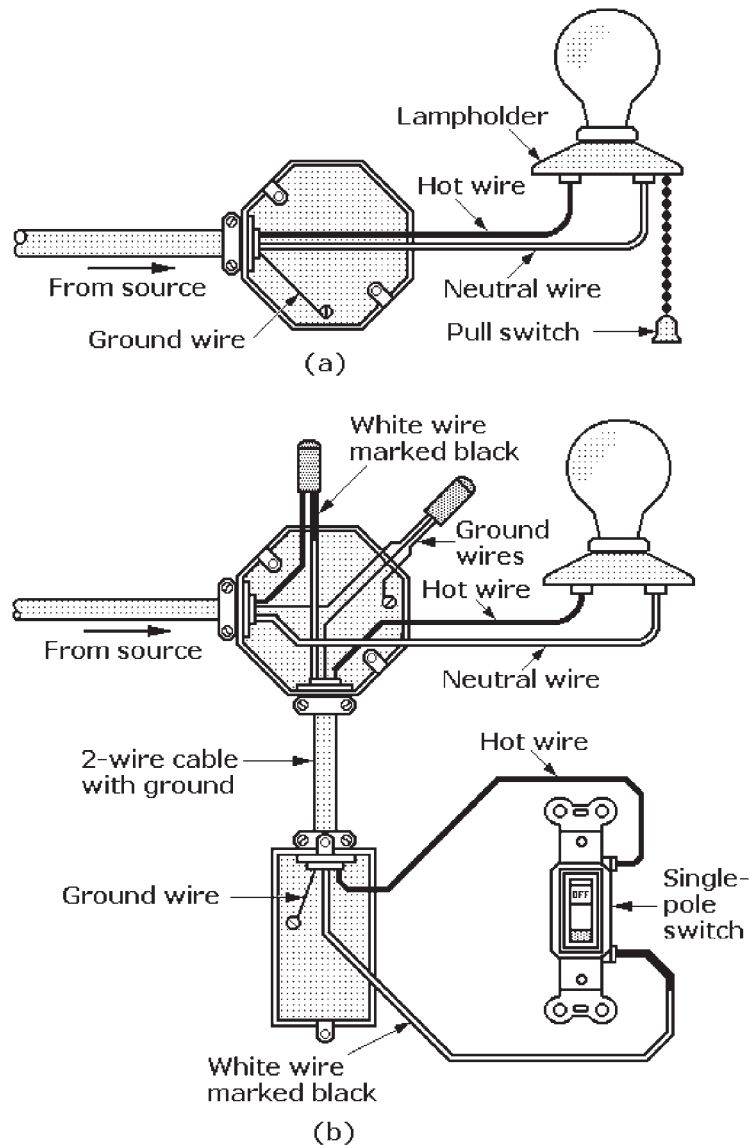
Figure 7-4 Lamps at the ends of circuits: (a) A circuit ends at a lampholder with a pull-chain switch; (b) a circuit with a lampholder at the end is controlled by a single-pole switch.
