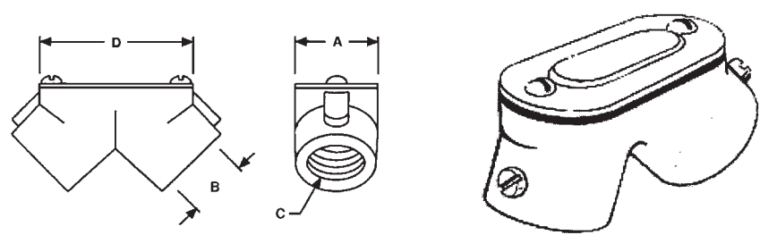
DIMENSIONS (inches)
