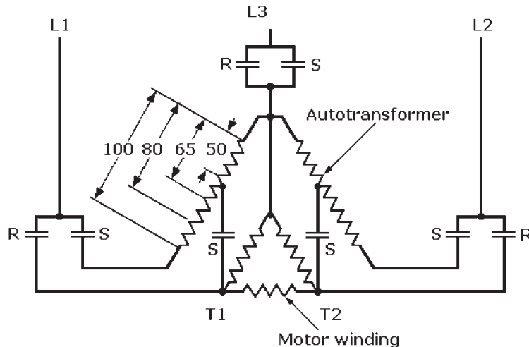
Figure 10-13 Automatic open-transition autotransformer motor starter.
