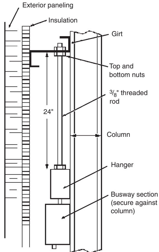
Figure 1-10 Electrical construction detail for hanging a busway.
