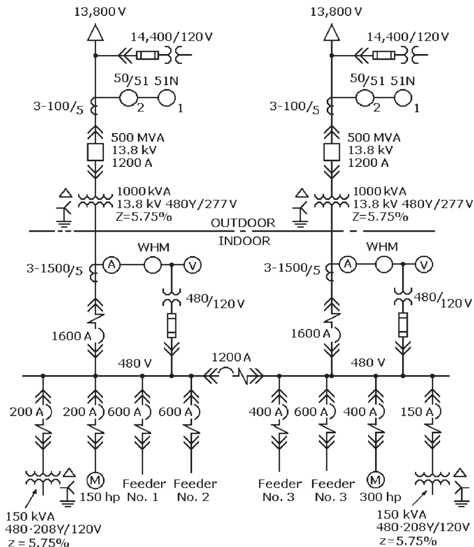
Figure 1-7 Typical one-line electrical diagram.
