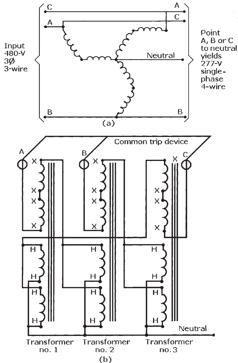
Figure 3-16 Auto zigzag grounding transformer: (a) for deriving a neutral; (b) wiring diagram.
