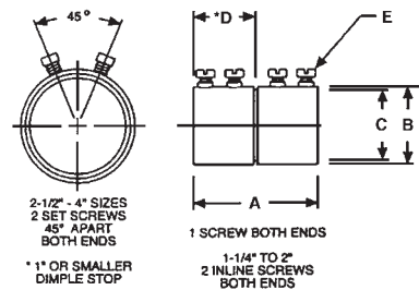
DIMENSIONS (inches)
