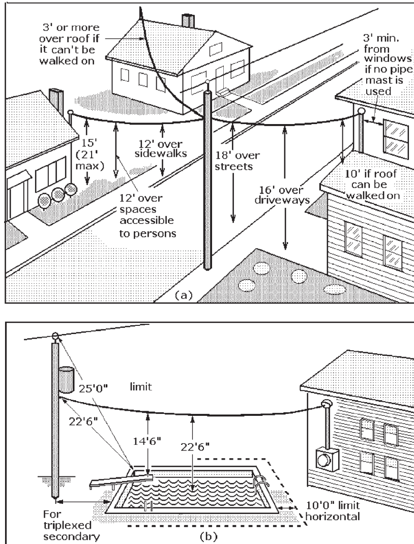
Figure 4-12 Clearance dimensions for service laterals: (a) typical residential situations; (b) over a swimming pool and accessories.
