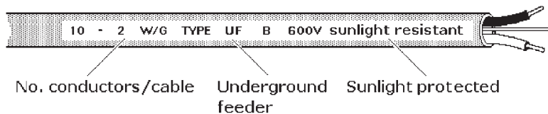
Figure 6-3 Codes printed on the jackets of cables identify them as: (a) service entrance (SE), (b) nonmetallic (NM), and (c) underground feeder (UF).
