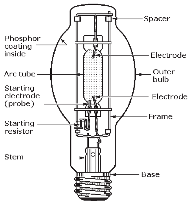
Figure 8-9 Mercury-vapor (MV) lamp construction.
