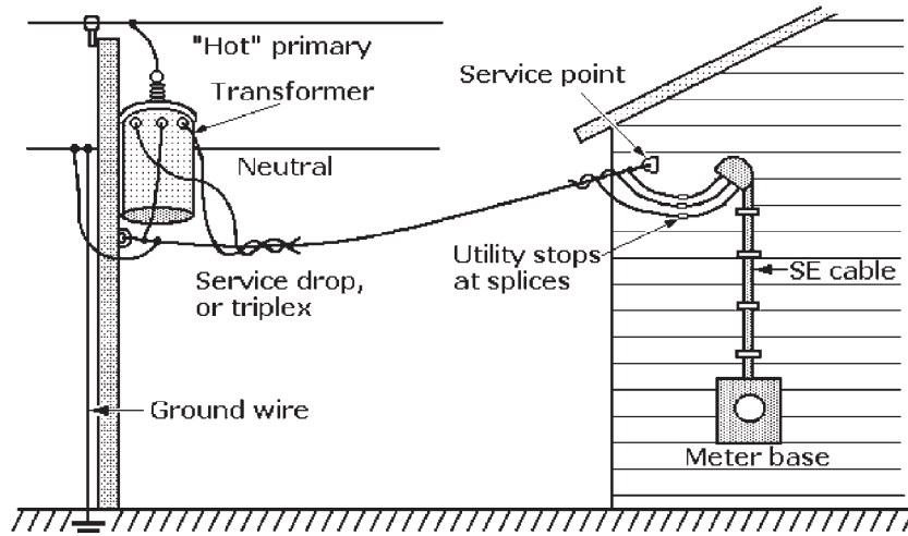
Figure 5-1 Overhead service provides electricity via a service drop from the utility pole transformer to the building service point.
