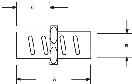
DIMENSIONS (inches)
