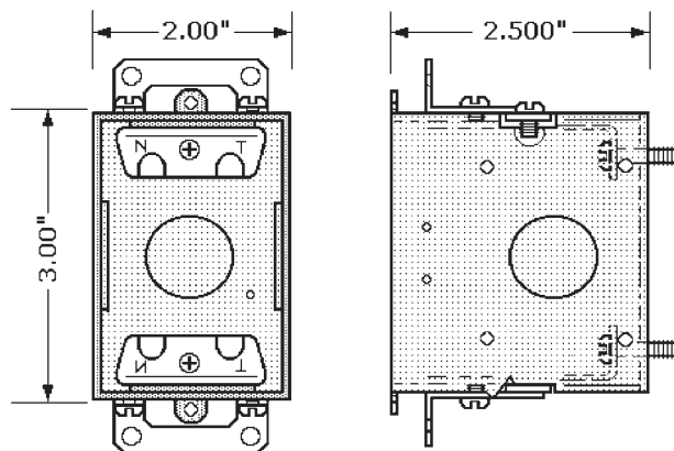
Figure 6-7 Metal 3-in. \times 2-in. gangable device box sized for a single switch or duplex receptacle has a volume of 12.5 in. 3 .
