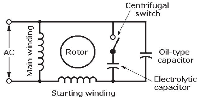
Figure 10-8 Two-capacitor start/one-capacitor run motor.
