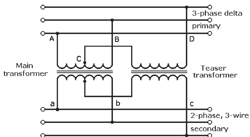
Figure 3-11 T-connected transformers.
