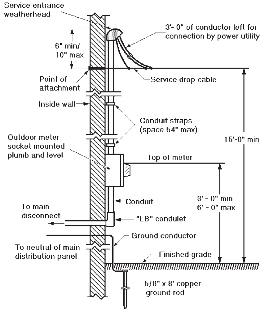
Figure 5-6 Riser layout for a typical overhead service entrance, giving dimensions and grounding details.
