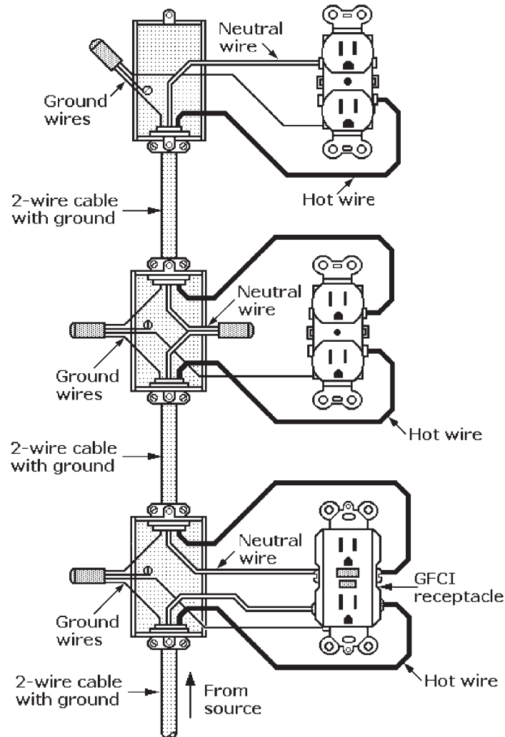
Figure 7-15 Duplex GFCI receptacle protects two downstream receptacles.
