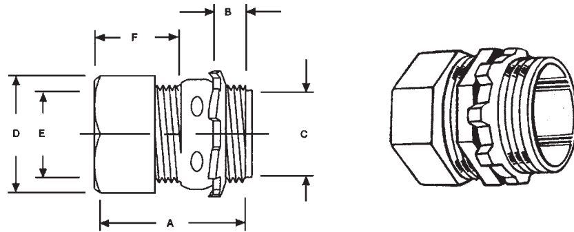
DIMENSIONS (inches)
