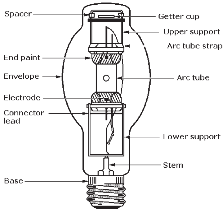
Figure 8-10 Metal-halide (MH) lamp construction.
