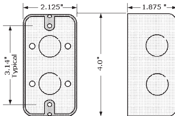
Figure 6-8 Metal utility 3-in. \times 2-in. device box has a volume of 13.0 in. 3 .
