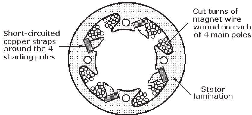
Figure 10-9 End view of the stator of a four-pole shaded-pole motor with four shading poles.
