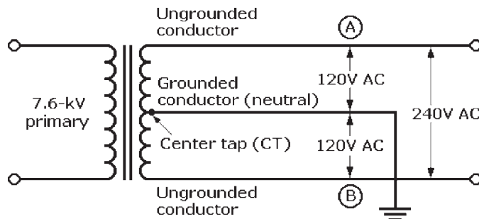
Figure 5-2 Single-phase distribution transformer steps 7.6 kV down to 240 V AC across the secondary winding; 120 V AC is obtained across both points A and B and the grounded conductor.
