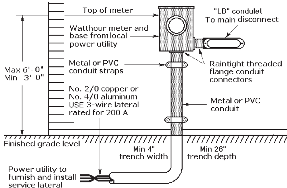
Figure 5-8 Underground service lateral rated for 200 A: layouts for 100 and 175 A are similar, but they have lower-rated underground service entrance (USE) cables.
