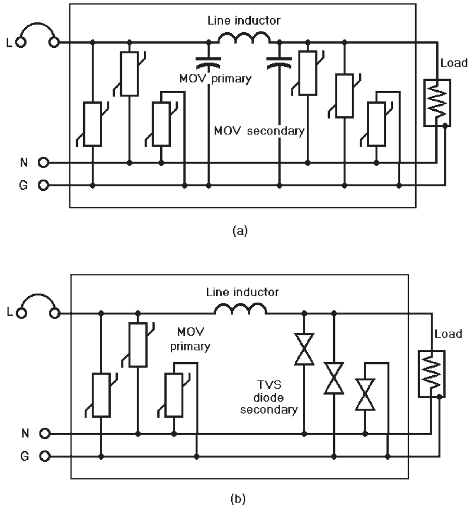
Figure 12-3 Surge protective device hybrid networks: (a) MOV primaries and secondaries; (b) MOV primaries and transient voltage suppressor (TVS) secondaries.
