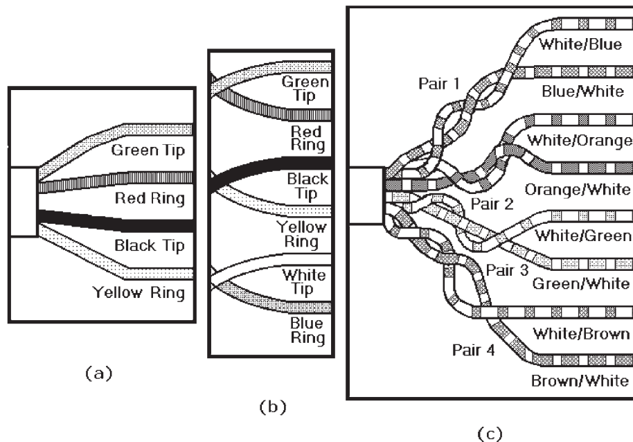
Figure 9-4 Telephone and multimedia cable: (a) solid-color, two-pair quad (nontwisted) phone; (b) solid-color, three twisted-pair phone; (c) band-striped, four twisted-pair multimedia.
